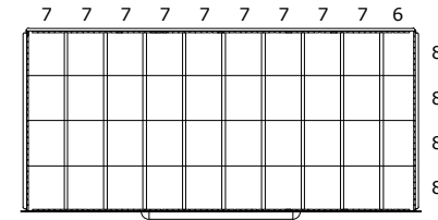
DRAWER LAYOUT "AS" 40 COMPARTMENTS
