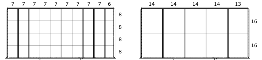
DRAWER LAYOUT "AS" 40 COMPARTMENTS
