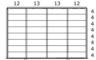
DRAWER LAYOUT "AJ" 32 COMPARTMENTS
