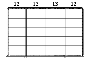
DRAWER LAYOUT "0K" 20 COMPARTMENTS
