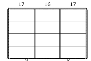
DRAWER LAYOUT "0L" 12 COMPARTMENTS
