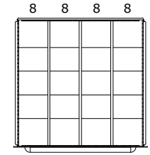
DRAWER LAYOUT "OK" 20 COMPARTMENTS
