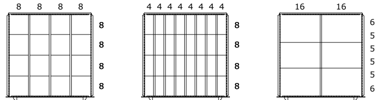
DRAWER LAYOUT "0P" 16 COMPARTMENTS DRAWER LAYOUT "0J" 32 COMPARTMENTS DRAWER LAYOUT "0M" 6 COMPARTMENTS
