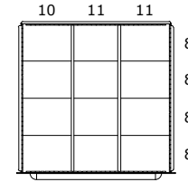
DRAWER LAYOUT "OL" 12 COMPARTMENTS
