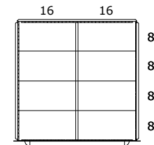
DRAWER LAYOUT "0D" 8 COMPARTMENTS
