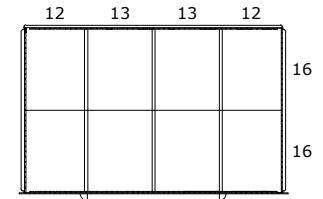
DRAWER LAYOUT "0D" 8 COMPARTMENTS
