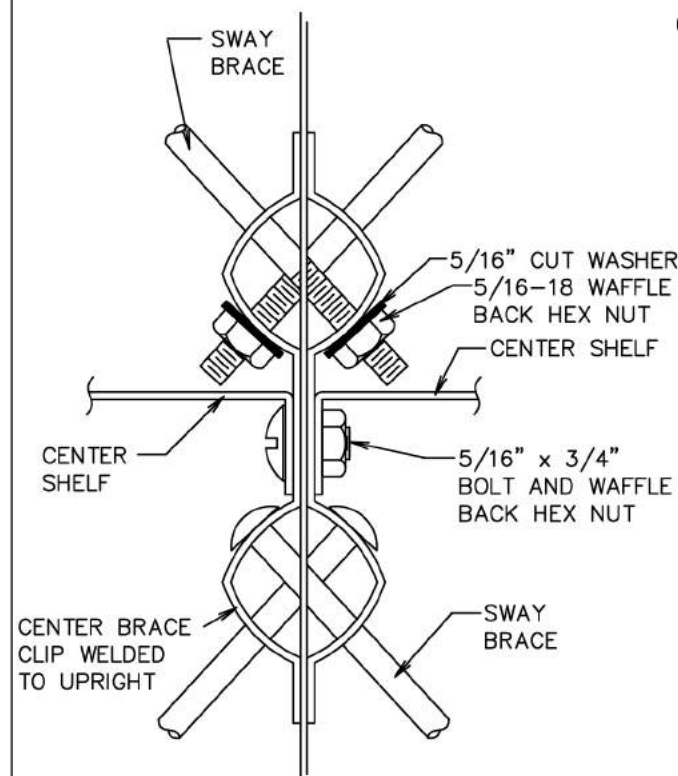
SECTION THROUGH UPRIGHT SHOWING ATTACHMENT OF SWAY BRACE.
