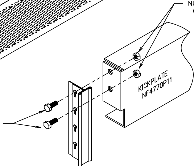
ASSEMBLY OF KICKPLATE TYP. FOR ALL
