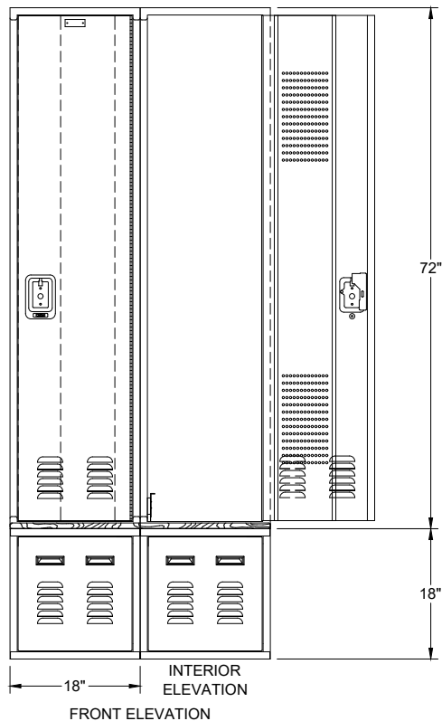
WELDED VALOR LOCKER FRAMES 18" X 24" X 72" S.R.S.T. W/ WELDED LOWER COMPARTMENT 18" X 36" X 18"
