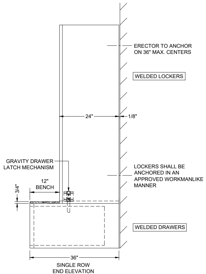
WELDED VALOR LOCKER FRAMES 18" X 24" X 72" S.R.S.T. W/ WELDED LOWER COMPARTMENT 18" X 36" X 18"
